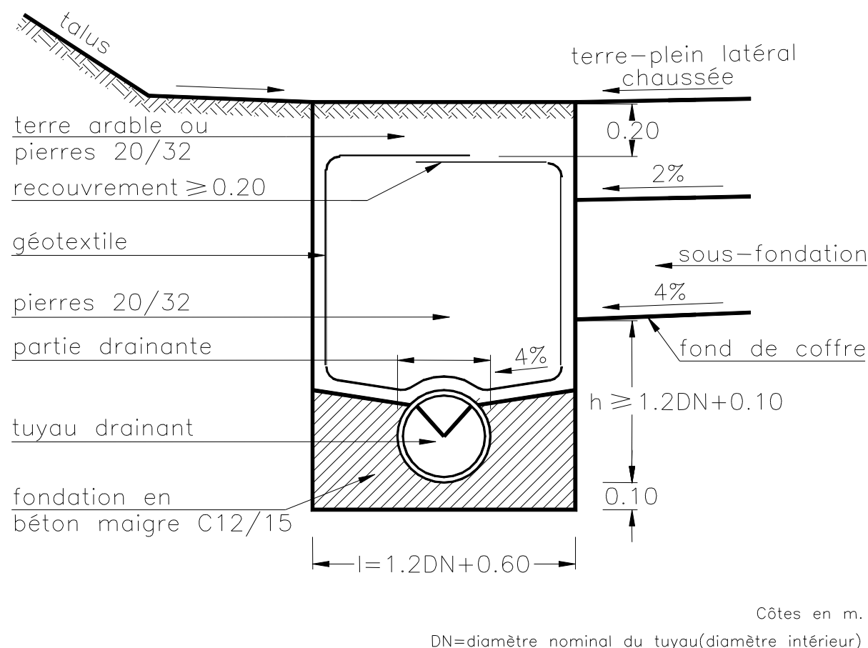
Fig.I.1.2.2.4. – AQUEDUC – DRAIN
